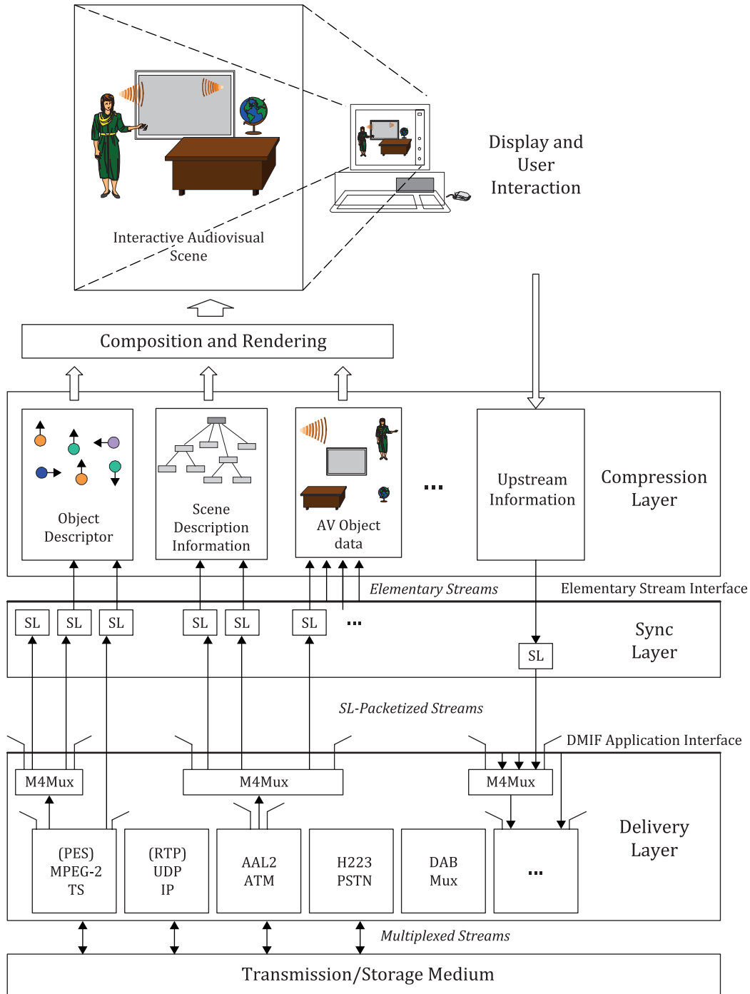
Figure 1 — The ISO/IEC 14496 series terminal architecture
